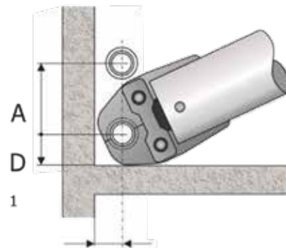
Figure 37 - Minimum distances and space requirements
