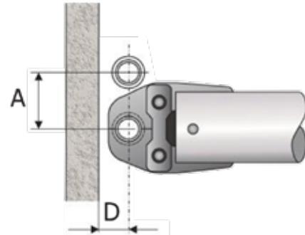
Figure 36 - Minimum distances and space requirements
